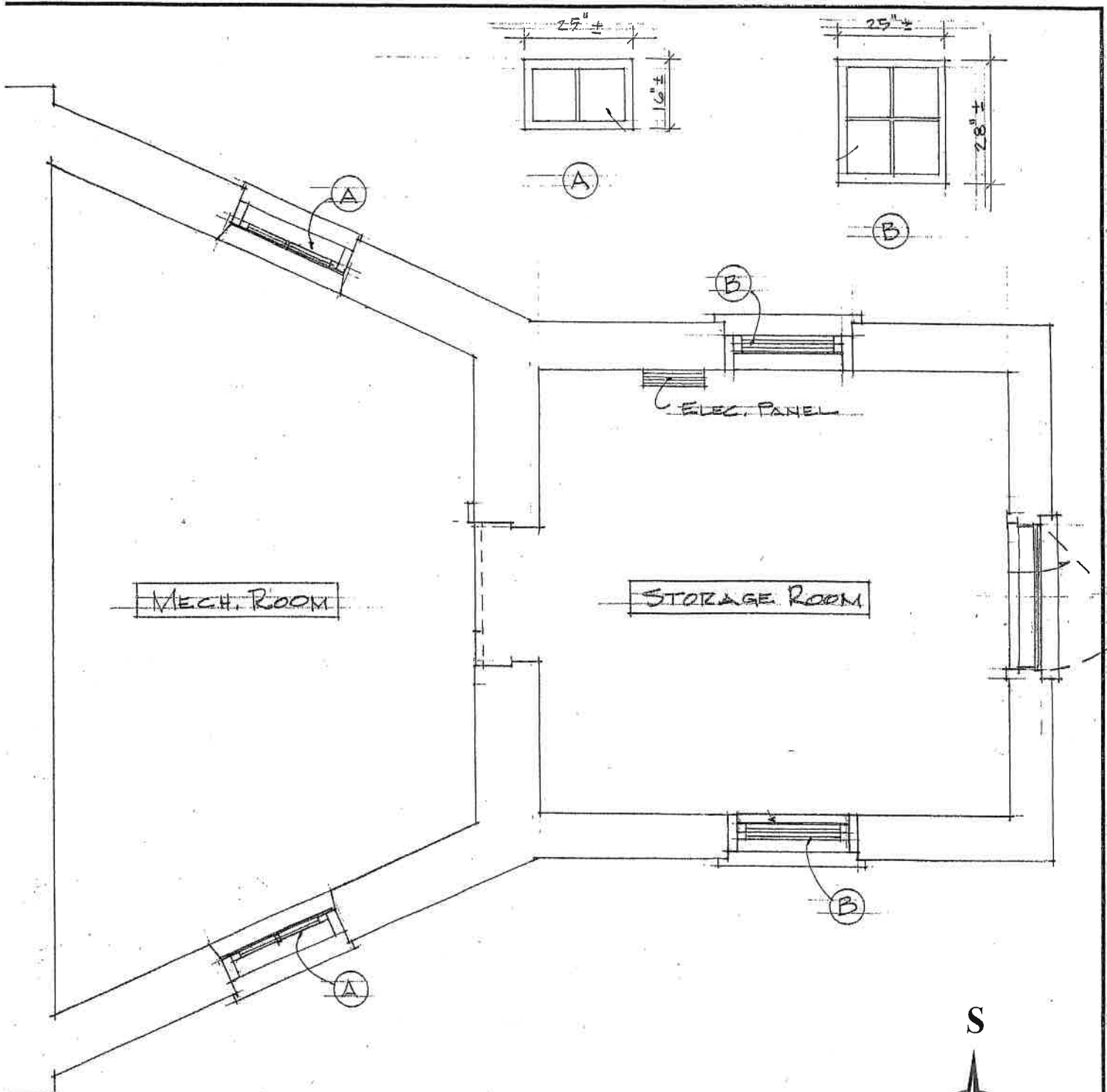
LOWER LEVEL PLAN SCALE: 3/8" = 1'-0"
